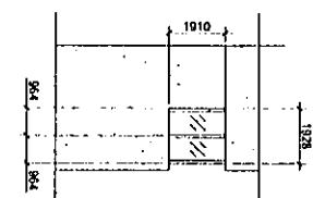
3 SIDE ELEVATION 1/8" = 1'-0"
