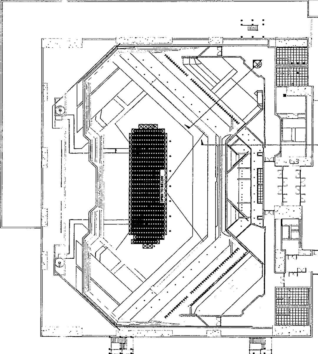
1 A13 SCALE 2ND FLOOR CEILING PLAN NT
