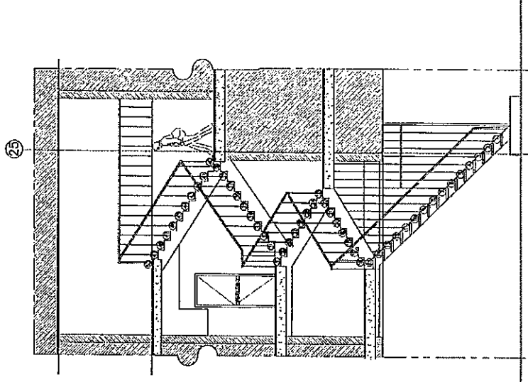
IMPROVEMENT OF EXISTING FIRE EXIT STAIR AT SECRETARIAT BLDG. SECTION A SCALE 1:30 MTS
