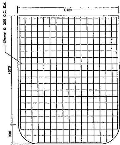
1 SLAB REINFORCEMENT DETAIL S-02 1/10
