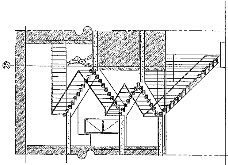
IMPROVEMENT OF EXISTING FIRE EXIT STAIR AT SECRETARIAT BLDG. SECTION A SCALE: 1/4" = 1'-0" 1/8" = 1'-0"
